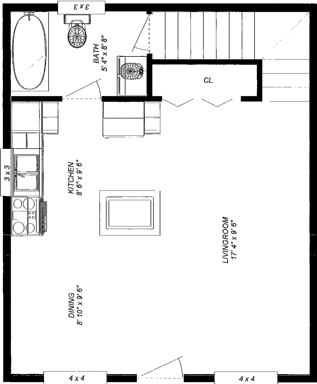
PLAN 10 20' x 24' 960 sq. ft. (1st Floor)
